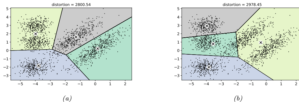
Figure 21.7: Illustration of K -means clustering in 2d. We show the result of using two different random seeds. Adapted from Figure 9.5 of [Gér19]. Generated by kmeans_voronoi.ipynb .
