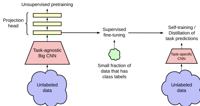
Figure 19.13: Combining self-supervised learning on unlabeled data (left), supervised fine-tuning (middle), and self-training on pseudo-labeled data (right). From Figure 3 of [Che+20c]. Used with kind permission of Ting Chen.
