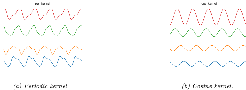
Figure 17.3: Functions sampled from a GP using various stationary periodic kernels. Generated by gpKernelPlot.ipynb .
