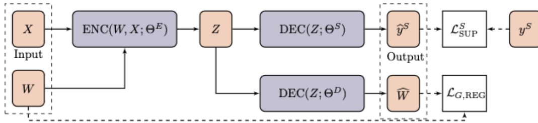
Figure 23.2: Illustration of the GRAPHEDM framework from Chami et al. [Cha+21]. Based on the supervision available, methods will use some or all of the branches. In particular, unsupervised methods do not leverage label decoding for training and only optimize the similarity decoder (lower branch). On the other hand, semi-supervised and supervised methods leverage the additional supervision to learn models' parameters (upper branch). Reprinted with permission from [Cha+21].
