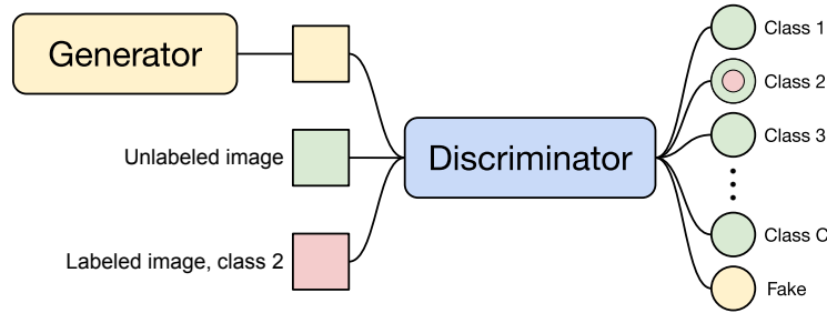
Figure 19.12: Diagram of the semi-supervised GAN framework. The discriminator is trained to output the class of labeled datapoints (red), a “fake” label for outputs from the generator (yellow), and any label for unlabeled data (green).
