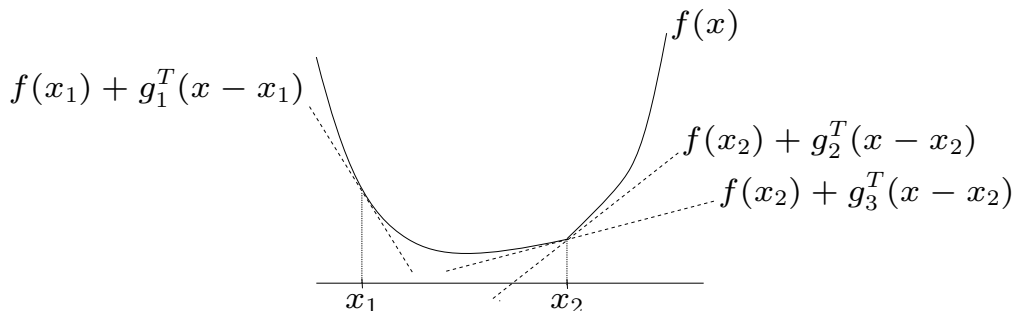
Figure 8.9: Illustration of subgradients. At x_1 , the convex function f is differentiable, and g_1 (which is the derivative of f at x_1 ) is the unique subgradient at x_1 . At the point x_2 , f is not differentiable, because of the “kink”. However, there are many subgradients at this point, of which two are shown. From https://web.stanford.edu/class/ee364b/lectures/subgradients_slides.pdf . Used with kind permission of Stephen Boyd.
