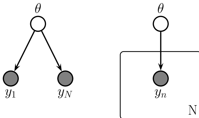
Figure 3.16: Left: data points \mathbf{y}_n are conditionally independent given \theta . Right: Same model, using plate notation. This represents the same model as the one on the left, except the repeated \mathbf{y}_n nodes are inside a box, known as a plate; the number in the lower right hand corner, N , specifies the number of repetitions of the \mathbf{y}_n node.
