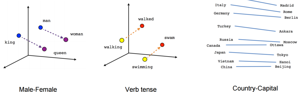
Figure 20.45: Visualization of arithmetic operations in word2vec embedding space. From https://www.tensorflow.org/tutorials/representation/word2vec .
