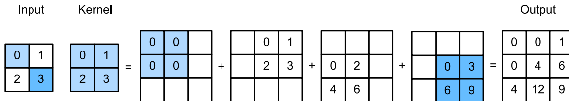
Figure 14.24: Transposed convolution with 2 \times 2 kernel. From Figure 13.10.1 of [Zha+20]. Used with kind permission of Aston Zhang.
