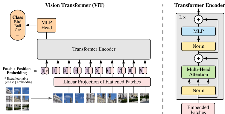
Figure 15.28: The Vision Transformer (ViT) model. This treats an image as a set of input patches. The input is prepended with the special CLASS embedding vector (denoted by * ) in location 0. The class label for the image is derived by applying softmax to the final output encoding at location 0. From Figure 1 of [Dos+21]. Used with kind permission of Alexey Dosovitskiy
